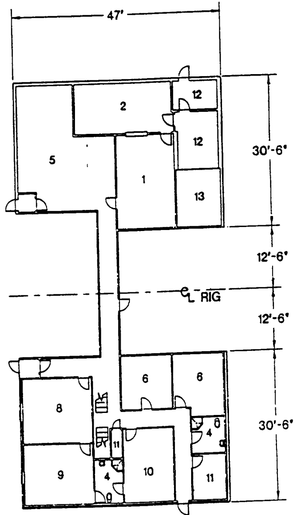
CAPACITY: (16) MEN MAIN DECK LEVEL
