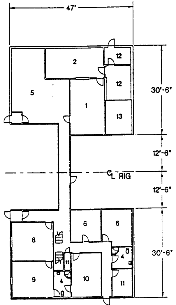
CAPACITY: (16) MEN MAIN DECK LEVEL
