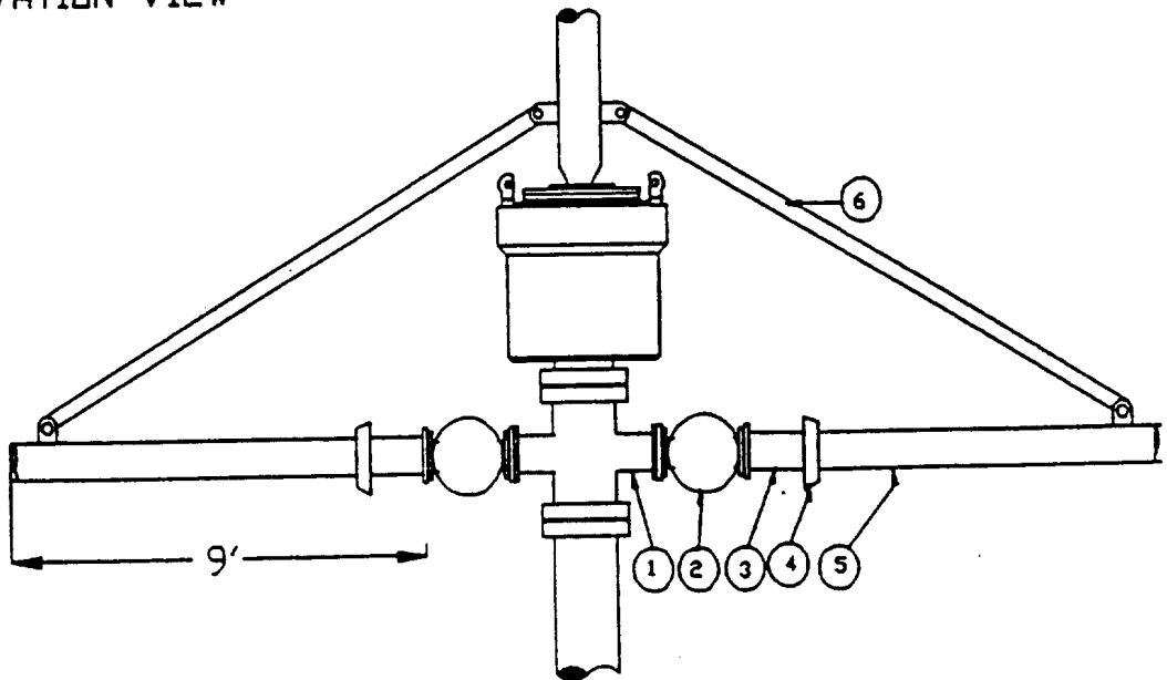
ELEVATION VIEW
