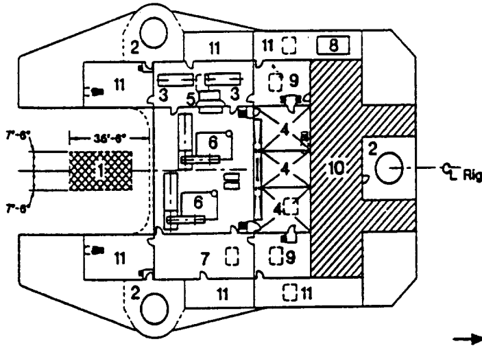
MACHINERY DECK
